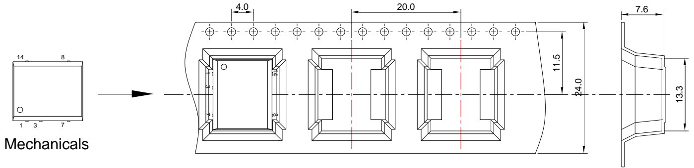
Tape & Reel
